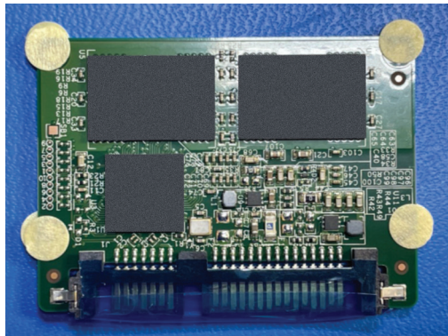
Figure 2: Example showing masking process to avoid seeping of conformal coating material into gold finger areas
